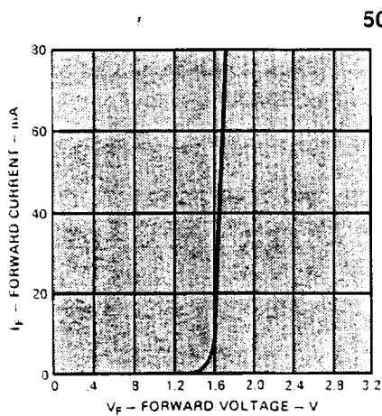
Figure 5. Forward Current vs. Forward Voltage.
